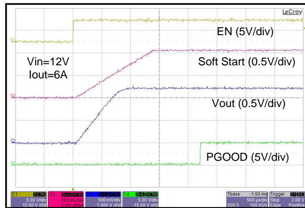
Figure 15. Startup Waveforms with 6 A Load Current
