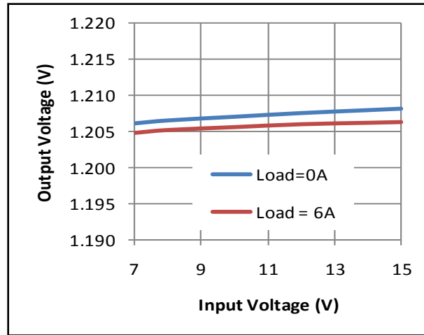
Figure 13. Line Regulation
